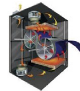
Through-Air Drum Drier Features Diagonally Offset Drums to increase Drying Area.
